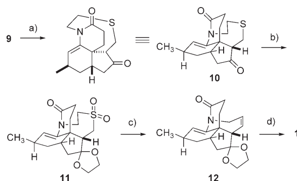
Scheme 5. Completion of the synthesis of 1 . Reagents and conditions: a) 1 M \text{NaOH} (76%); b) 1. ethylene glycol, \text{PPTS} , benzene (87%); 2. m\text{CPBA} , \text{CH}_2\text{Cl}_2 (98%); c) \text{CBr}_2\text{F}_2 , \text{KOH} -alumina, t\text{BuOH} , \text{CH}_2\text{Cl}_2 (46%); d) 1. \text{H}_2 , \text{Pd/C} , \text{EtOH}/\text{THF} (57%); 2. \text{LiAlH}_4 , \text{THF} (71%); 3. 1 M \text{HCl} , \text{THF} (60%). m\text{CPBA} = meta -chloroperbenzoic acid, \text{PPTS} = pyridinium para -toluenesulfonate.
